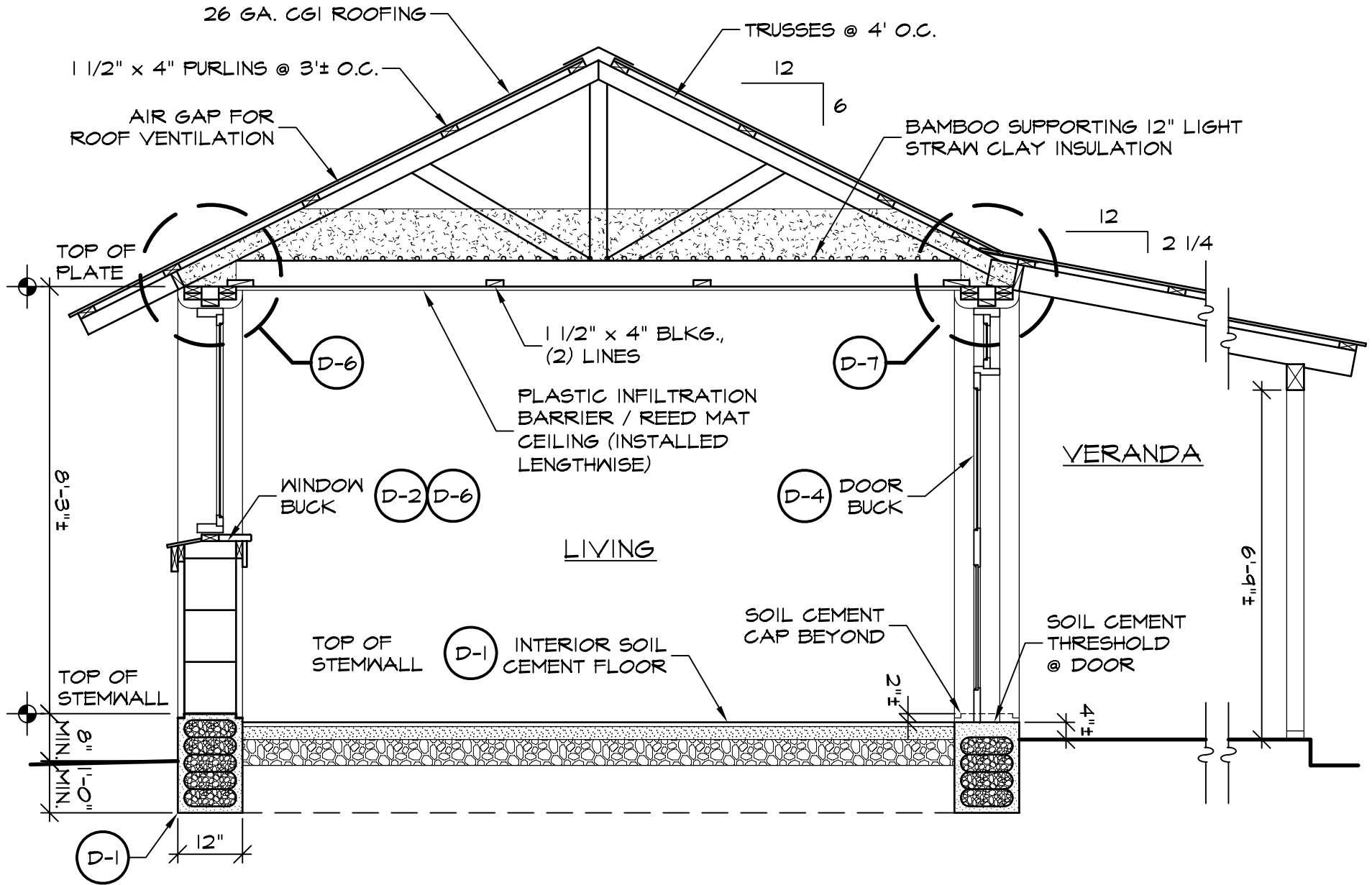
SECTION A 3/8" = 1'
