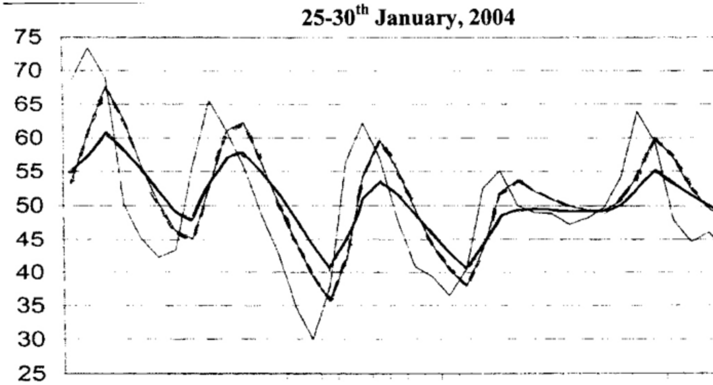
Figure 2a. Temperature data loggings during a cold period (25th to 30th of January 2004). The solid bold line represents adobe; the dashed line represents cinder block and the solid light line represents ambient temperature. Note that for every temperature extremes the cinder block had temperatures higher and lower than the adobe. Also fluctuation of temperature was greater for the cinder block than for the adobe.
