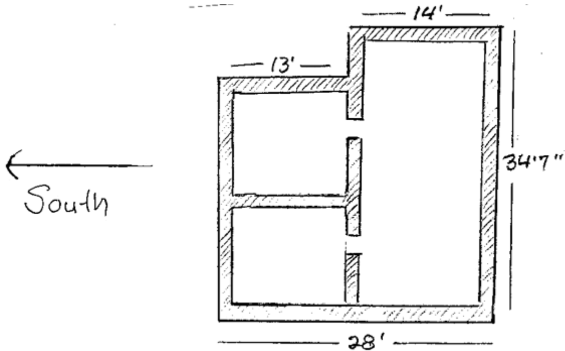
Figure 7. Original floor plan as of June 14, 1976. No insulation was used and no cooling mechanisms or overhangs existed. There was one window on the north side. Late in the day a large tree partially shaded the northwest corner of the house. The building was kept closed during the period the data was gathered.
